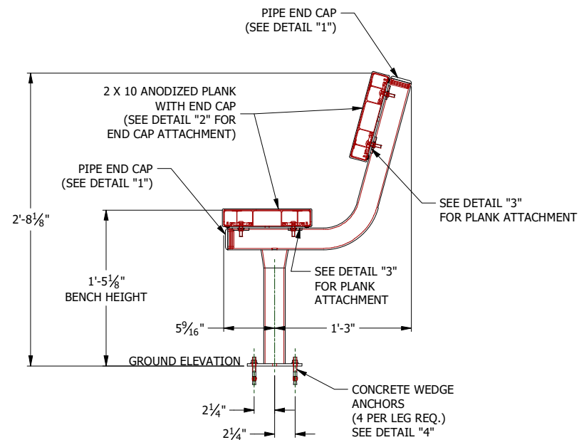
END VIEW
